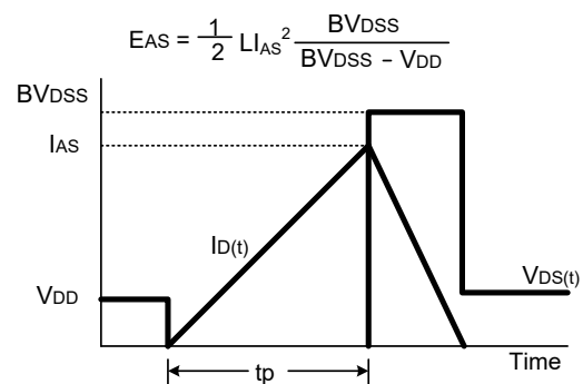
E_{AS} Test Circuit & Waveform
